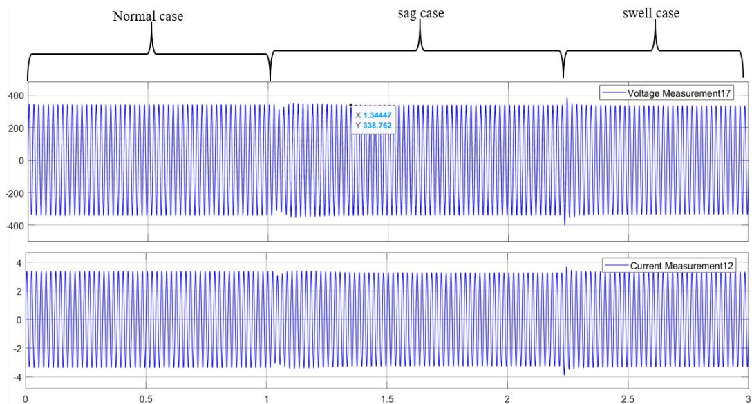
Figure 4. The voltage and current waveform in different conditions of the proposed converter.
