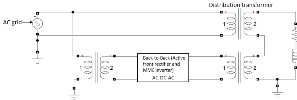
Figure 1. The proposed back-back converter in the primary side of the DT.
