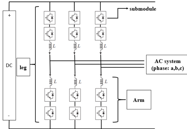
Figure 2. Circuit configuration of the MMC.
