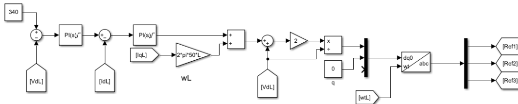
Figure 3. The proposed control of the MMC.
