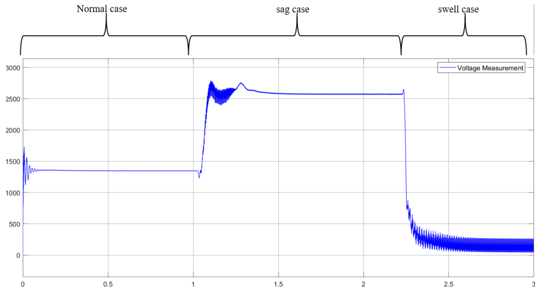
Figure 5. The DC-link of the proposed converter in different conditions.
