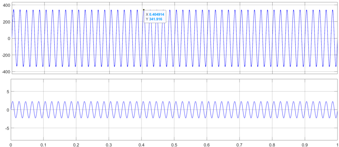
Figure 8. The output voltage and current waveform of the load resistor of 150\Omega .
