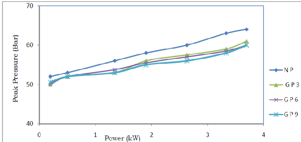
Fig. 3.4 Comparison of Peak pressure with different configurations of piston Source: S.L.V. Prasad et al. 2011
