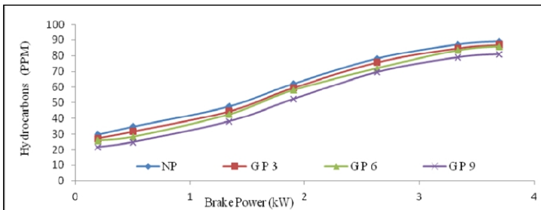
Fig. 3.5 Comparison of hydrocarbons with different configurations of piston Source: Bharathi et al. 2011
