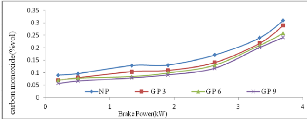
Fig. 3.6 Comparison of Carbon monoxide with different configurations of piston Source: Bharathi et al. 2011
