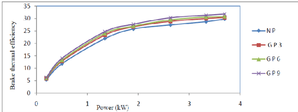
Fig. 3.1 Comparison of brake thermal efficiency with different configurations of piston Source: S.L.V. Prasad et al. 2011
