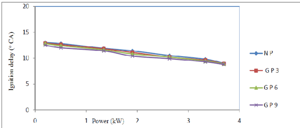
Fig. 3.3 Comparison of Ignition delay with different configurations of piston Source: S.L.V. Prasad et al. 2011
