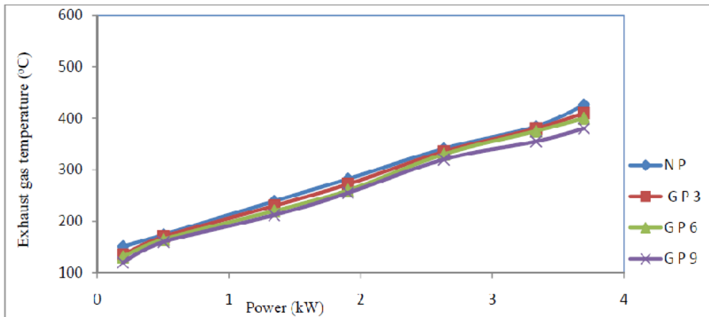
Fig. 3.2 Comparison of exhaust gas temperatures with different configurations of piston Source: S.L.V. Prasad et al. 2011
