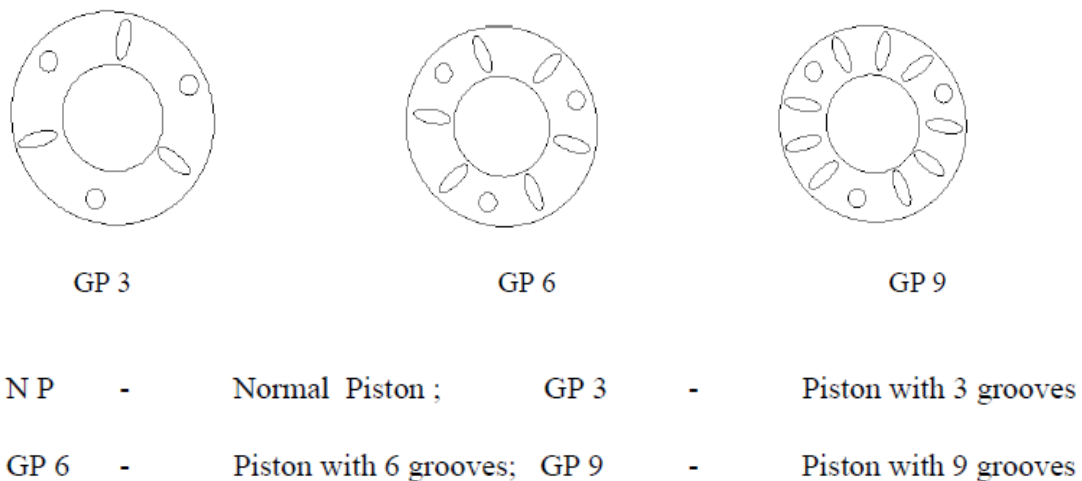
Fig. 2.1 Different types of configurations of piston crowns Source: S.L.V. Prasad et al. 2011
