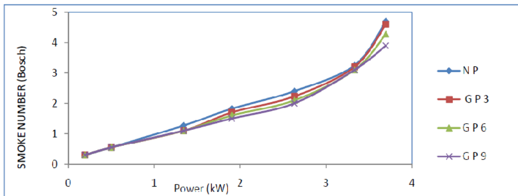
Fig. 3.7 Comparison of smoke densities with different configurations of piston Source: S.L.V. Prasad et al. 2011
