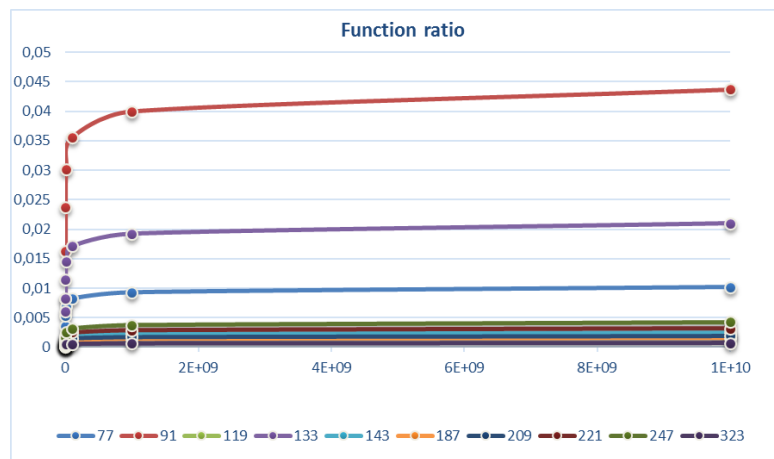
Figure 5. Function ratio (dependence on the boundary X , practical/theoretical).
