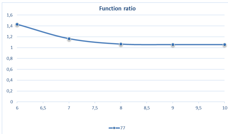
Figure 10. Function ratio (dependence on the logarithm of boundary X , practical/theoretical).
