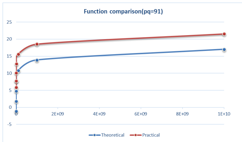
Figure 7. Comparison of theoretical and practical evaluation (dependence on the boundary X , pq=91 ).
