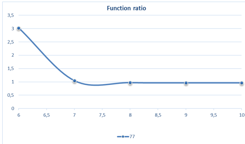
Figure 9. Function ratio (dependence on the logarithm of boundary X , practical/theoretical).
