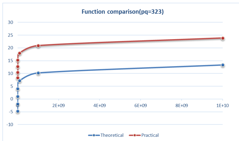
Figure 8. Comparison of theoretical and practical evaluation (dependence on the boundary X , pq=323 ).
