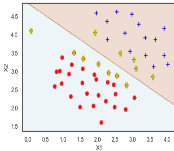
Figure 7. w_2 = \frac{1}{2}, w_1 = \frac{1}{2}, \alpha = 1 , number of support vectors = 12
