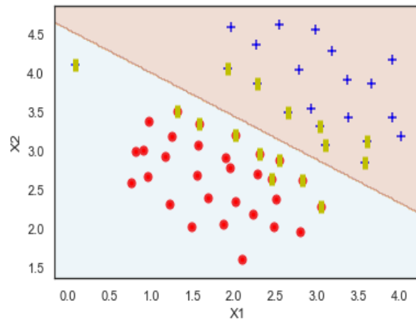
Figure 6. w_2 = \frac{1}{2}, w_1 = \frac{1}{2}, \alpha = \frac{1}{2} , number of support vectors = 16
