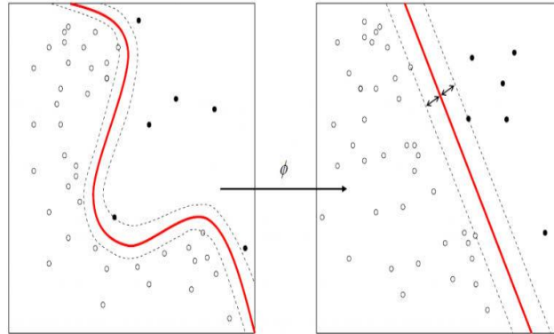
Figure 3. Linearly separable and nonlinearly separable
