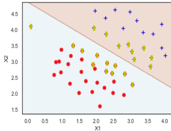
Figure 5. w_2 = \frac{1}{2}, w_1 = \frac{1}{2}, \alpha = \frac{1}{4} , number of support vectors = 20
